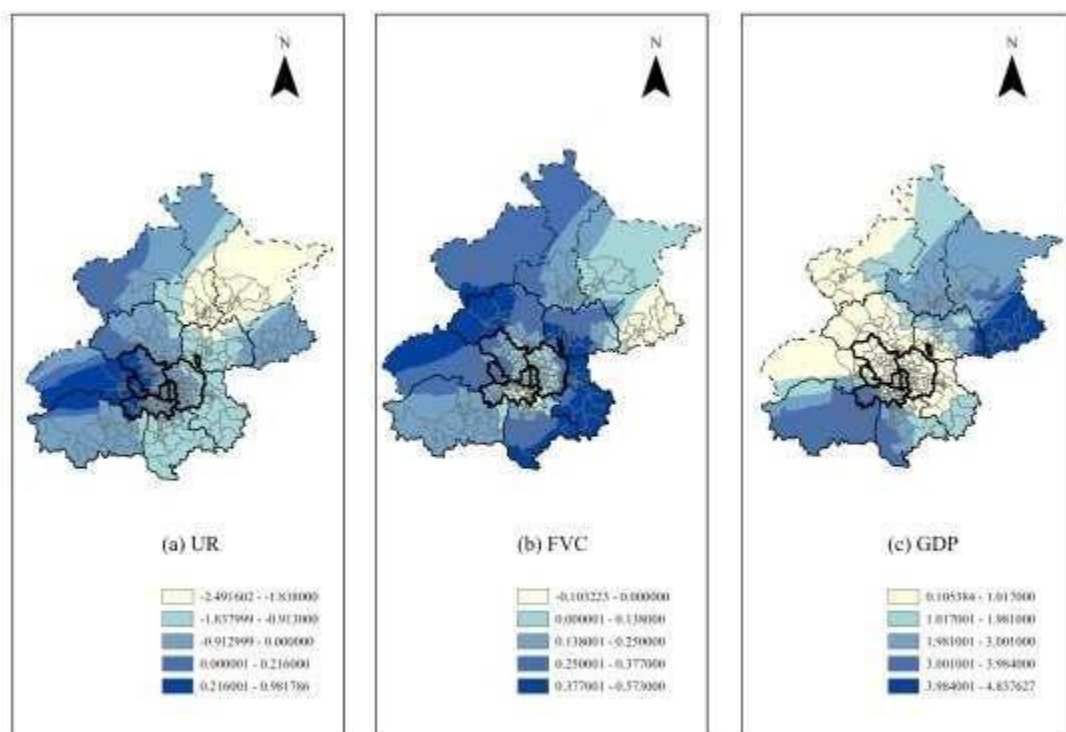
Figure 6: Displays the estimated coefficients for each spatial factor indicator across the study area.
